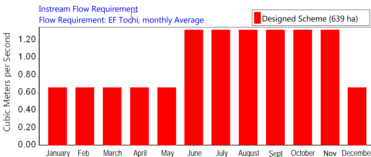
Figure 9.3 - Monthly environmental flow requirement (m 3 /s)
