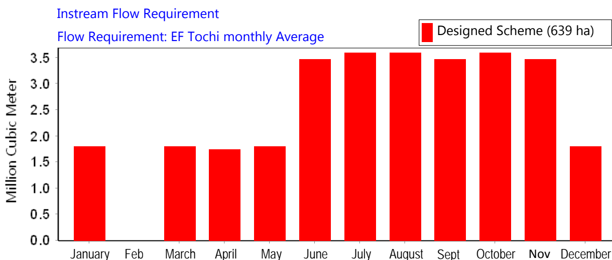
Figure 9.4 - Total monthly environmental flow requirement (Mm3)
