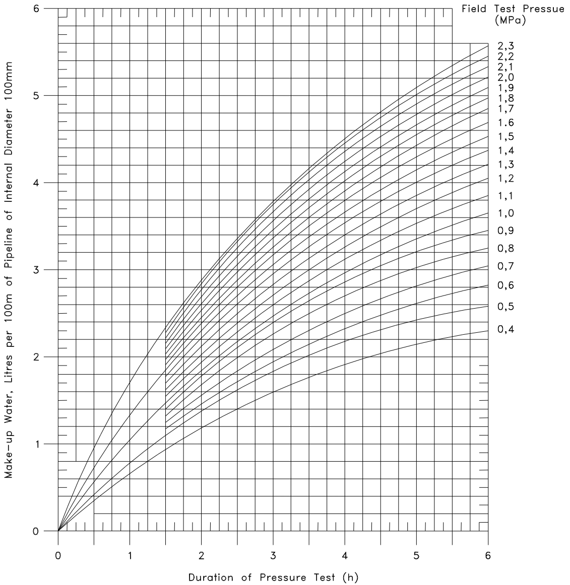
Figure D1: Make-up water in field testing of pressure pipes
