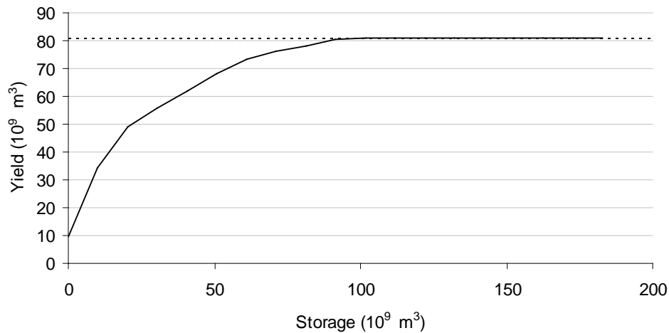
FIGURE 4B-3 STORAGE YIELD CURVE FOR THE NILE RIVER AT ASWAN
