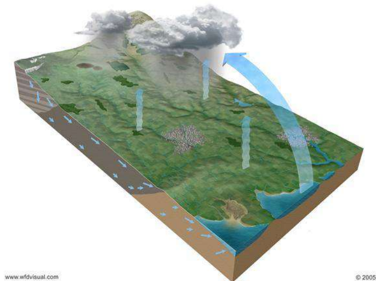
Figure 1: Water Cycle
