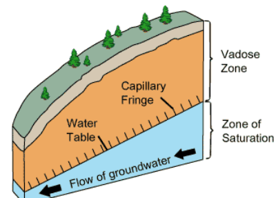
Figure 7: Illustration of the Vadose Zone (US Geological Survey)
