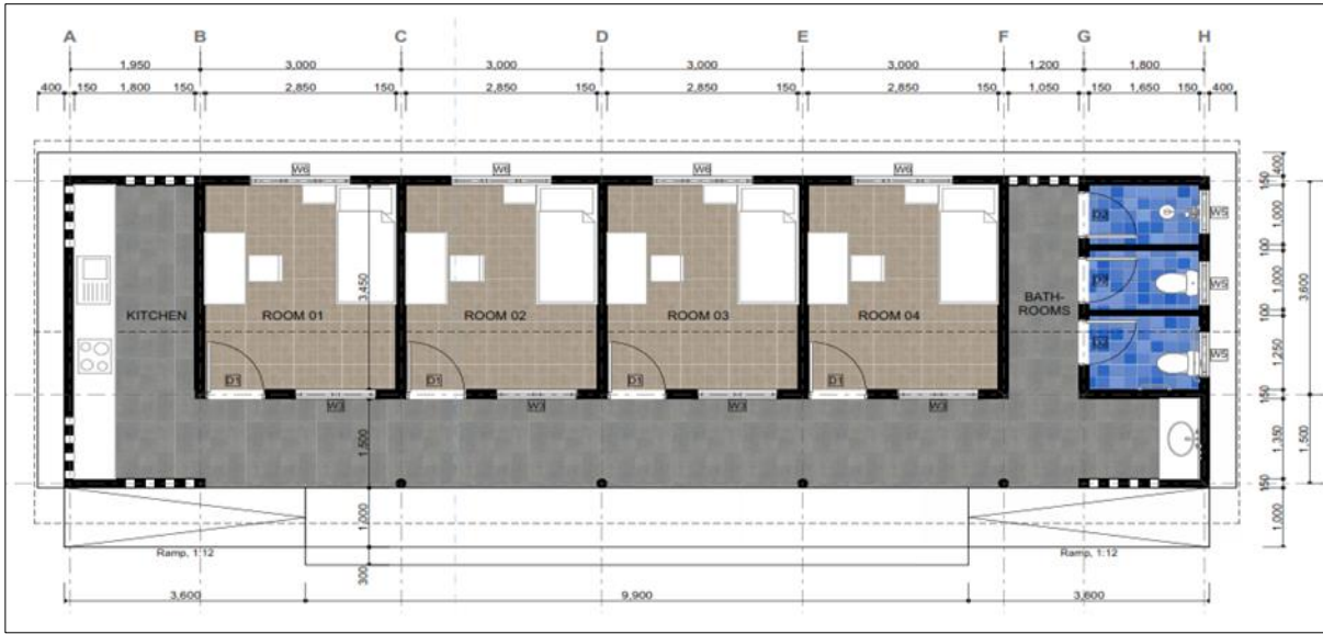
Figure 6: Security housing Floor Plan Design
