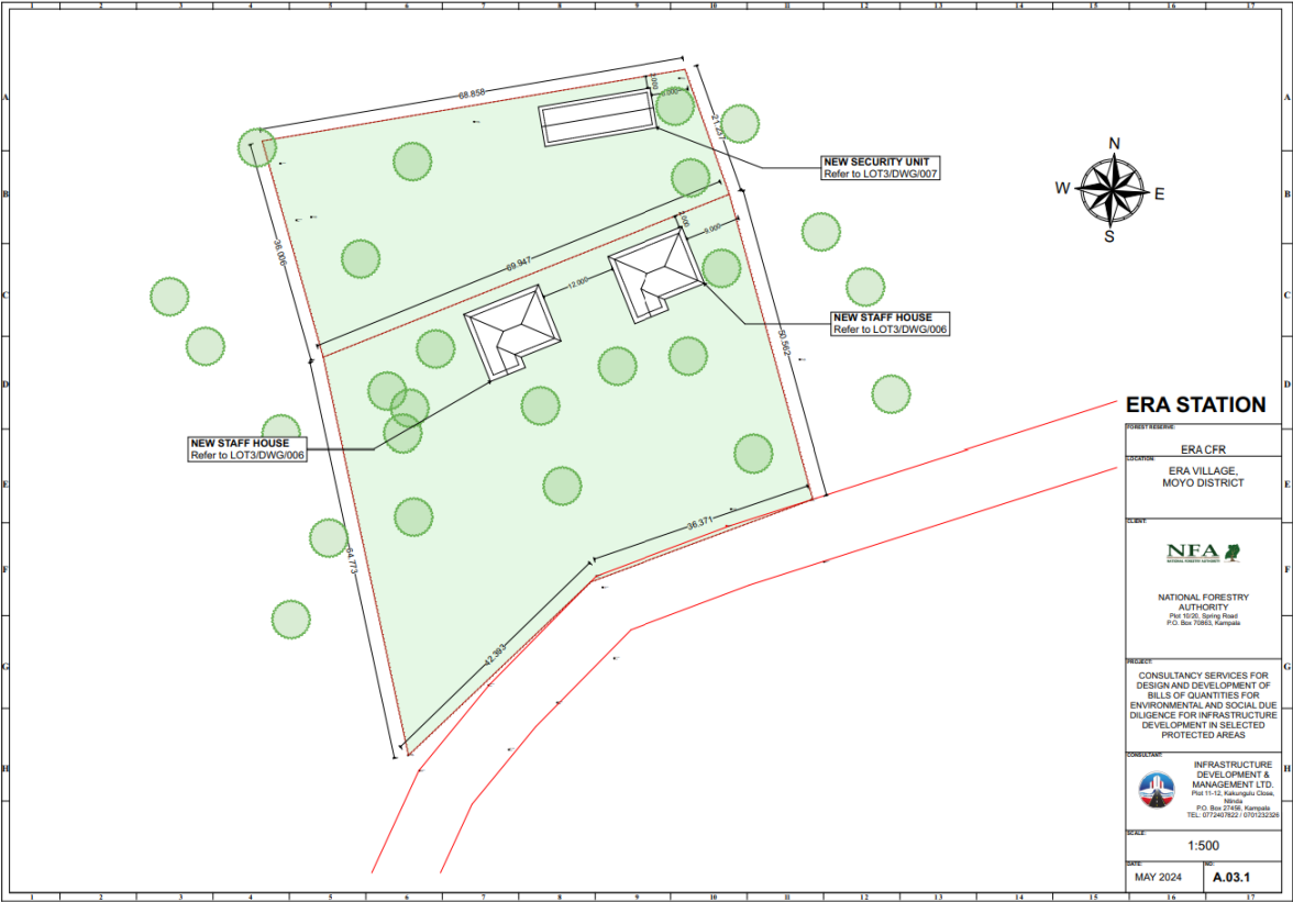
Figure 7: Era Site layout Plan
