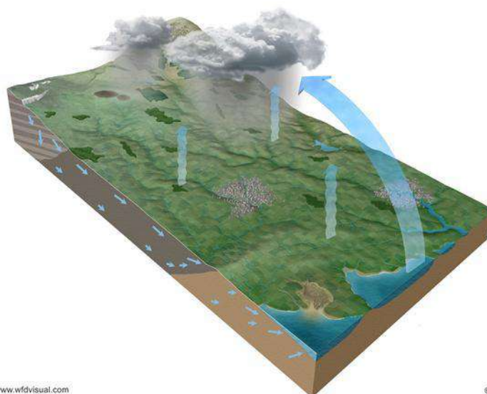
Figure 1: Water Cycle
