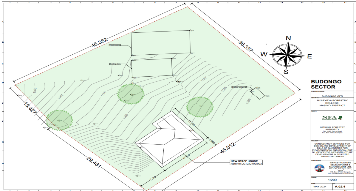
Figure 7: Nyabyeya office Site layout Plan
