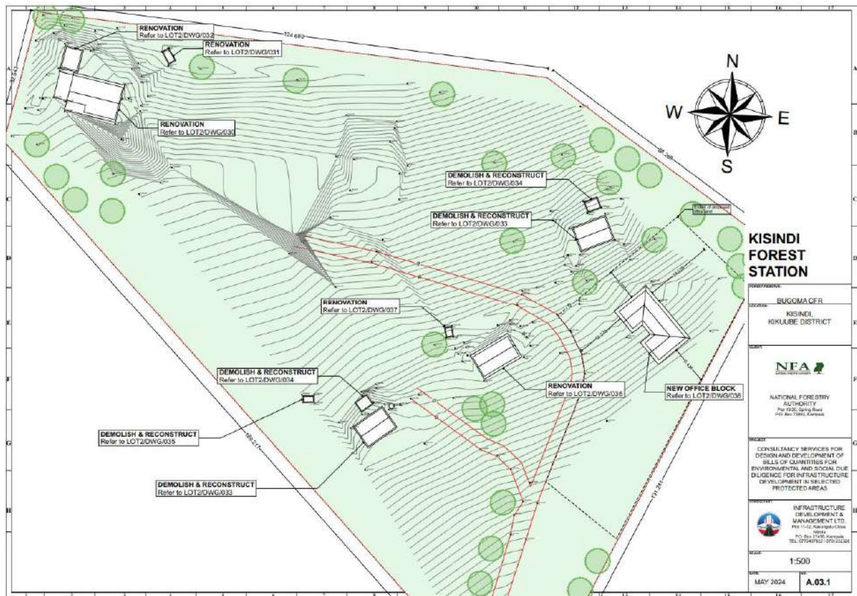
Figure 5: Bugoma site plan
